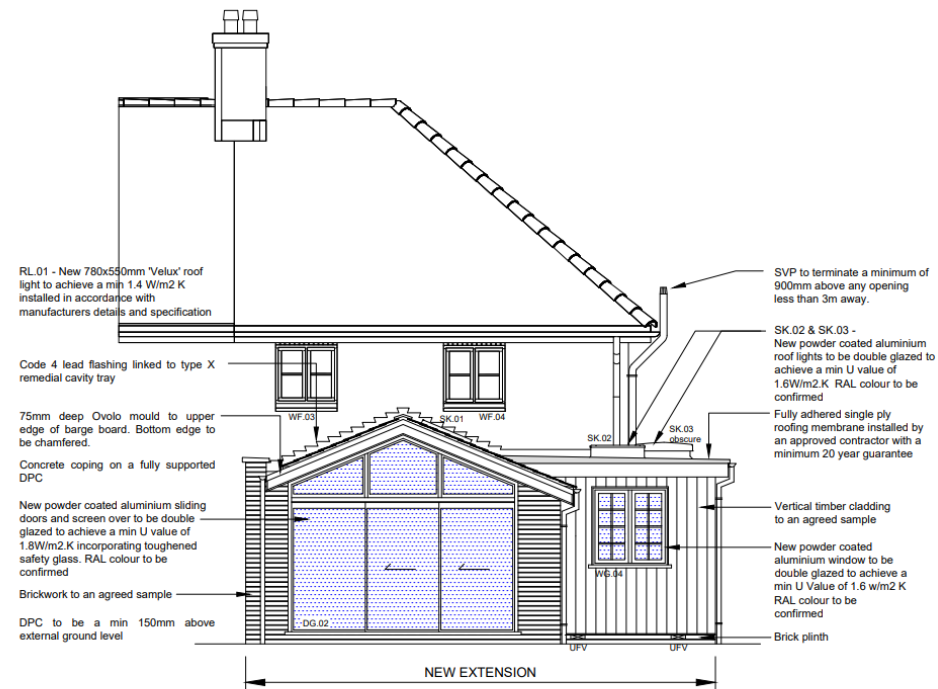
PROPOSED REAR ELEVATION @ 1:50
