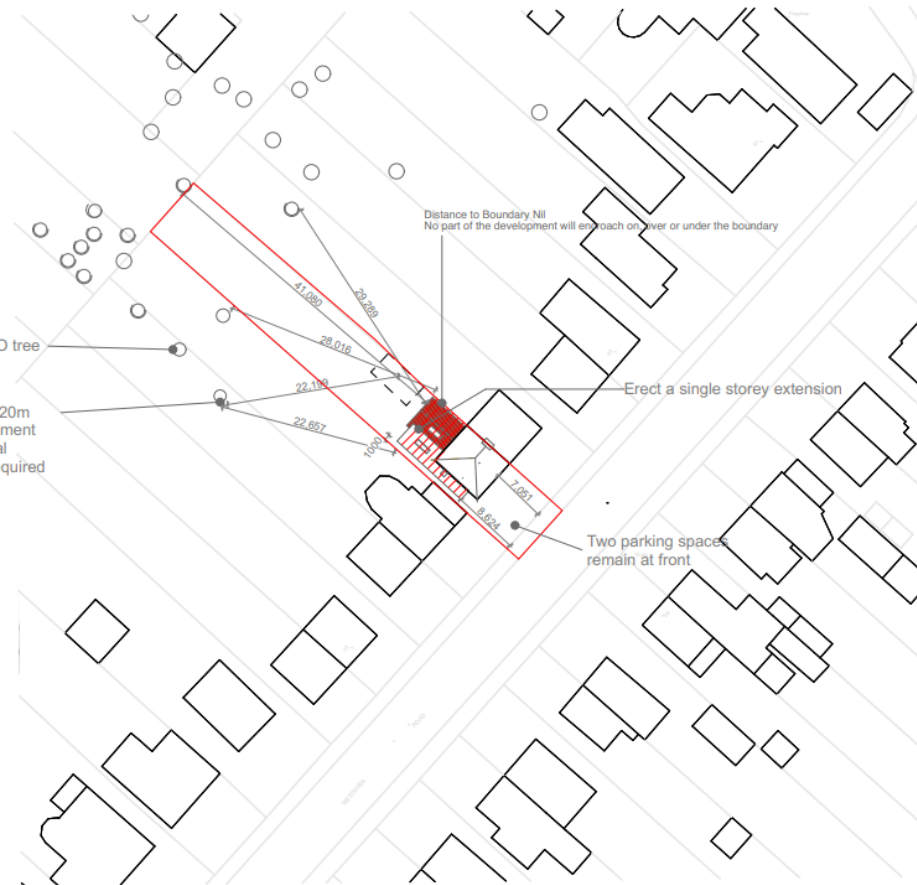
Block plan scale 1:500 ©Crown Copyright and database rights 2021 OS Licence no. 100019980
