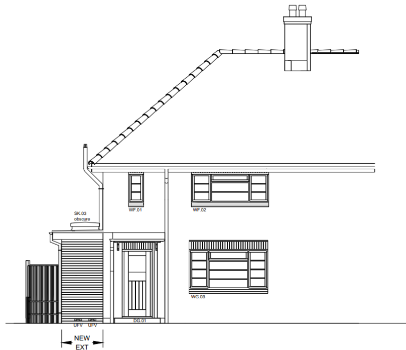
PROPOSED FRONT ELEVATION @ 1:50
